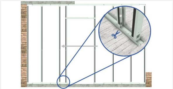
Door shifts to the left: this causes the I-module to the left of the door to protrude into the doorway. This piece must be cut off before the module is installed.
