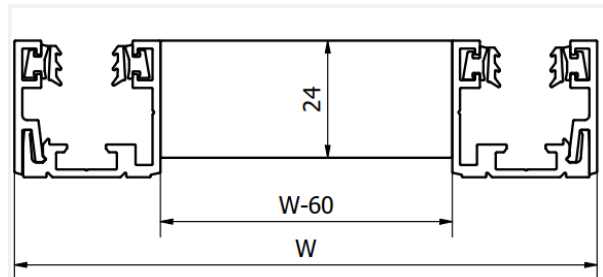
Double glass profile W = variable, min. 60 mm.
