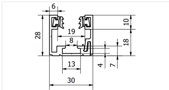
Single glass profile
