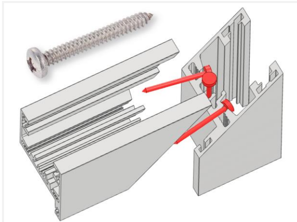
Connecting with screws
