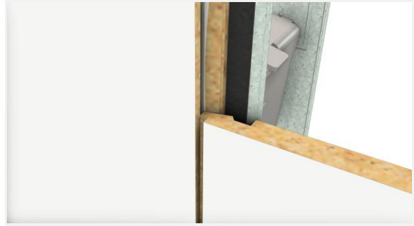
The cut groove allows the tongue of the 3 rd panel to slide sideways into the 2 nd panel. This requires a 3 mm clearance around the pipe itself.
